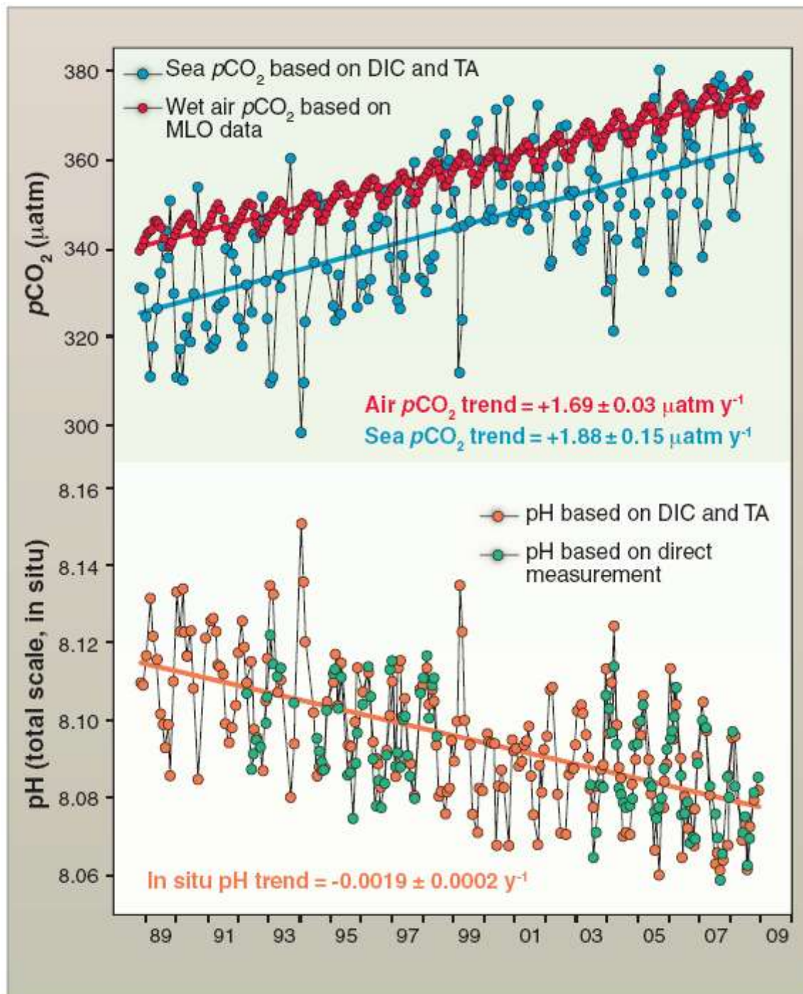
Fig. 2. Time series of (top) atmospheric CO 2 and surface ocean pCO 2 and (bottom) surface ocean pH at the atmospheric Mauna Loa Observatory (MLO) on the island of Hawai'i and Station ALOHA in the subtropical North Pacific north of Hawai'i, 1988–2008. [Adapted from (26)]
